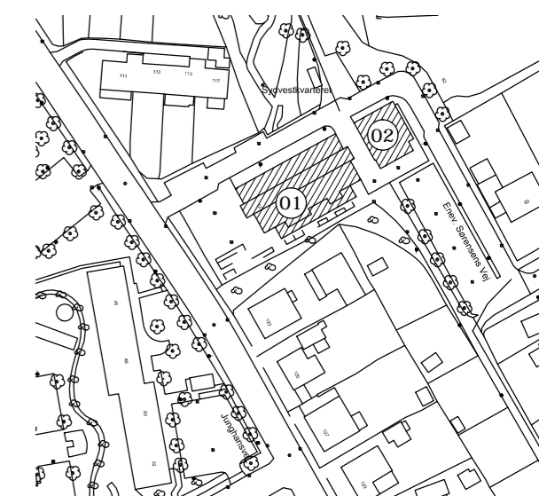
Situationsplan 1:2000
